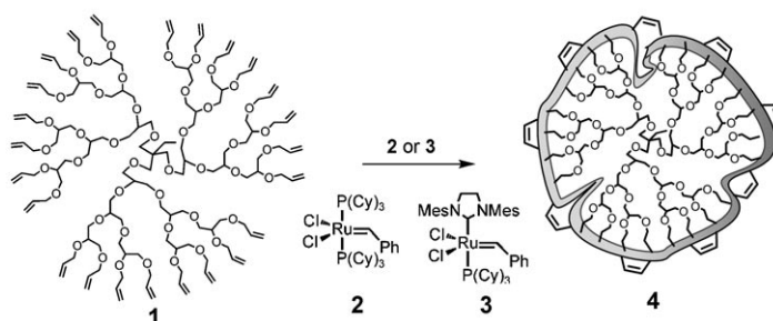
Scheme 1. RCM-mediated cross-linking of dendrimer 1 . Cy = cyclohexyl, Mes = 2,4,6-trimethylphenyl.
